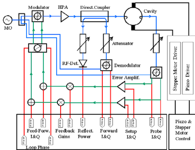
Figure 1: Low Level RF block-diagram.
