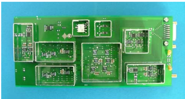
Figure 2: Low Level RF print board. The covers of the electromagnetic shields of individual sections are removed
