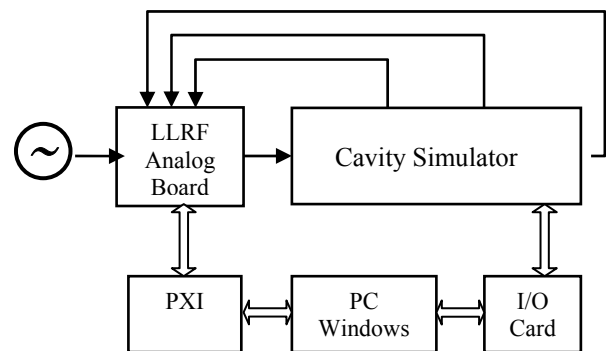
Figure 5: Block diagram of Low Level RF test assembly.
