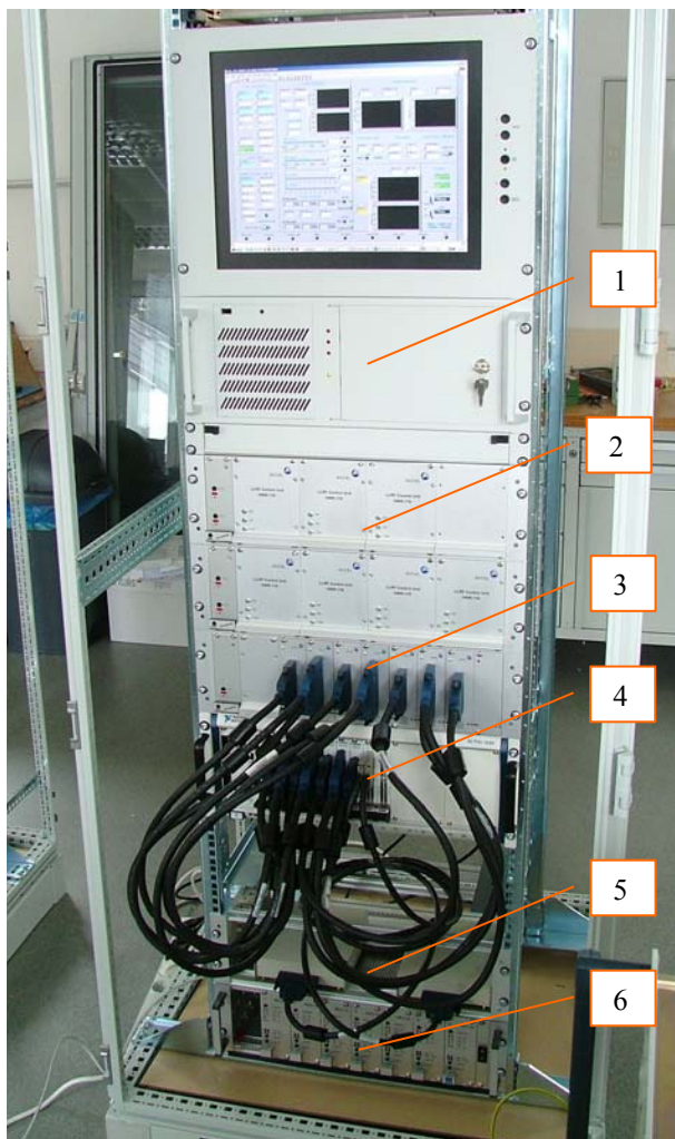
Figure 4: Low Level RF Control Rack. See text above for the legend.
